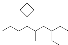
6-cyclobutyl-3-ethyl-5-methylnonane
