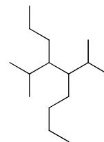
5-sec-butyl-4-isopropylnonane
