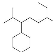
3-cyclohexyl-2,6-dimethyloctane
