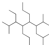
3-ethyl-6-isopropyl-2,8-dimethyl-4,5-dipropylnonane
