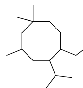
6-ethyl-5-isopropyl-1,1,3-trimethylcyclooctane
