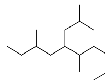
5-isobutyl-3,6-dimethyldecane
