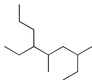
6-ethyl-3,5-dimethylnonane
